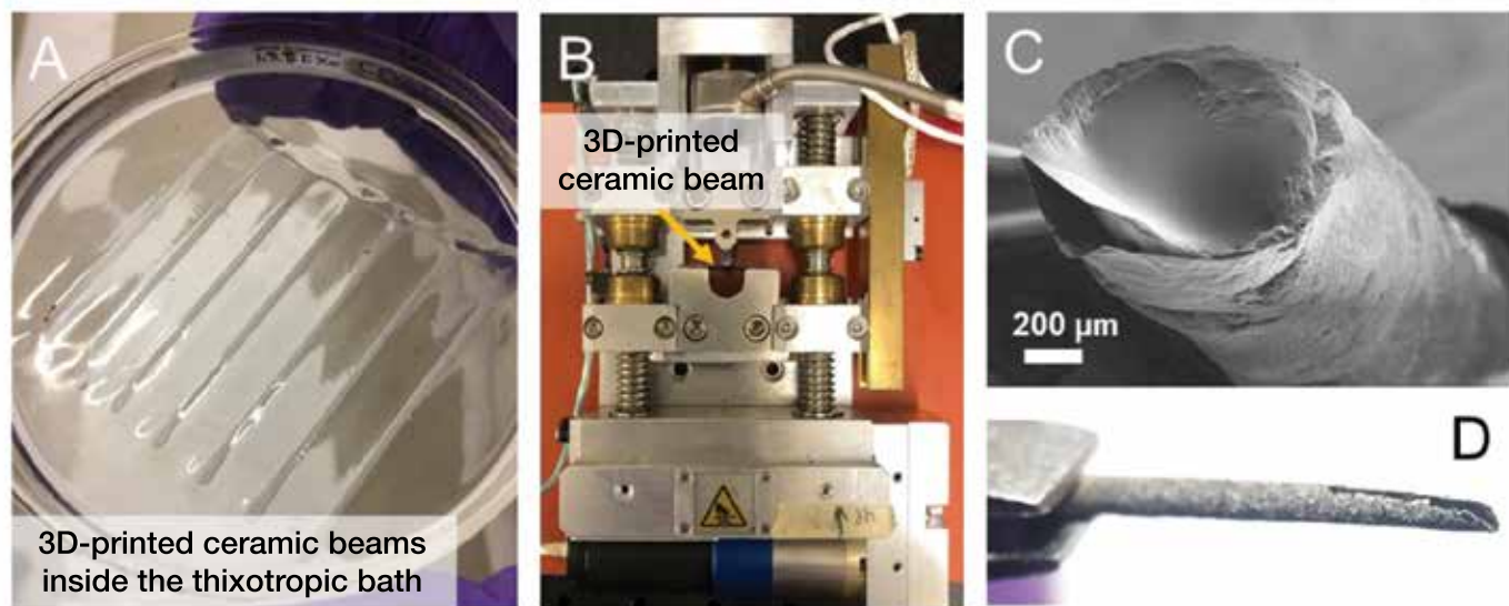
Figure 3. (A) Several 3D-printed ceramic beams inside the bath. The beams are as-printed (pre-crosslinking). (B) A pyrolyzed beam under three-point bending test. (C) A scanning electron microscope image of the cross-section of the beam after three-point bending test. (D) One piece of the broken beam after three-point bending test.
