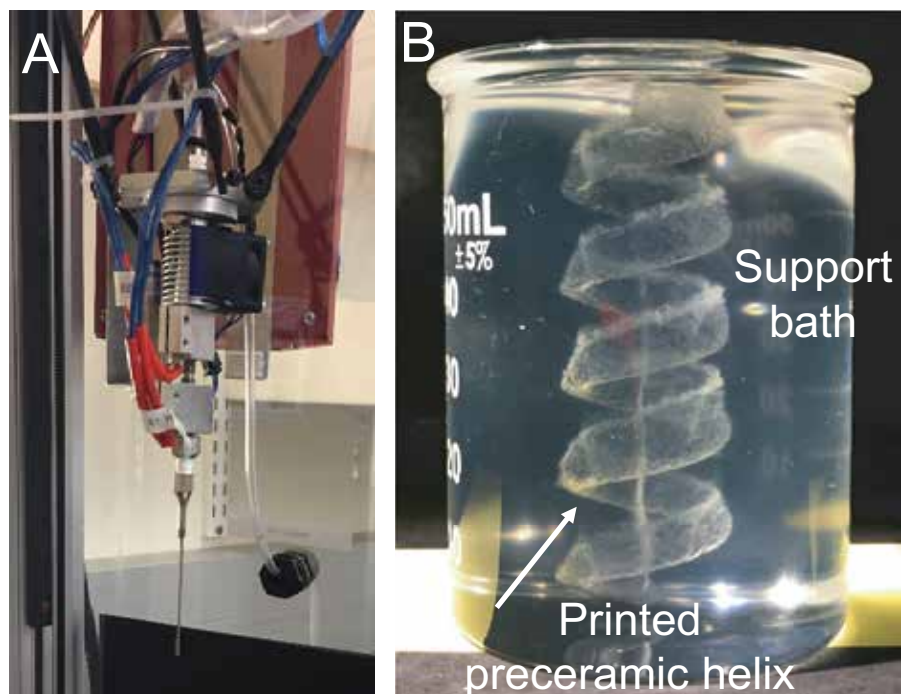
Figure 1. (A) The printhead with a long nozzle used for printing PDCs. (B) A close-up view of a helix printed inside the thixotropic bath.
