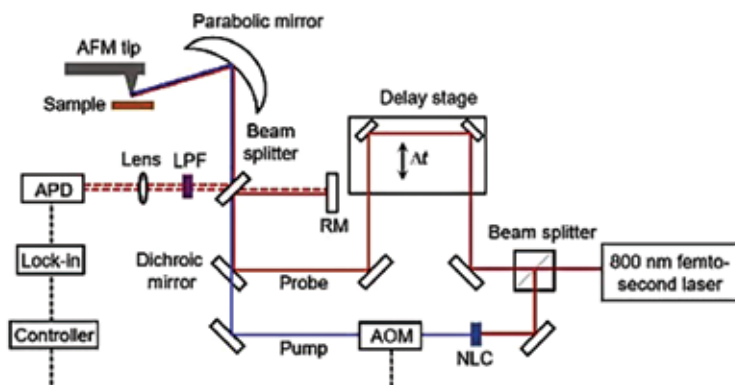
Experimental setup of the new optical nanoscopy system. NLC: non-linear crystal; AOM: acoustic-optic modulator; APD: avalanche photodiode; LPF: long-pass filter; RM: reference mirror. Reprinted with permission from Li et al., Nano Letters . Copyright 2023 American Chemical Society.
