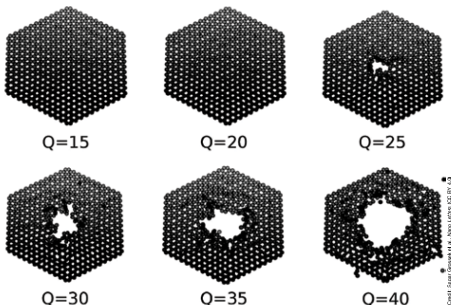
Restructuring of carbon layers due to the impact of a highly charged ion with initial charges ( Q_{in} ) ranging from 15–40 for a fixed hopping time of 7 au. The threshold for pore formation at this charge mobility is around Q_{in} = 25 .
